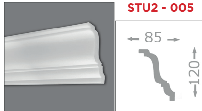
2000 x 85 x 120 mm / Polystyrol
