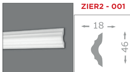
2000 x 18 x 46 mm / Polystyrol
