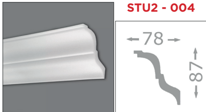
2000 x 78 x 87 mm / Polystyrol
