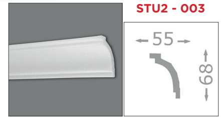
2000 x 55 x 68 mm / Polystyrol
