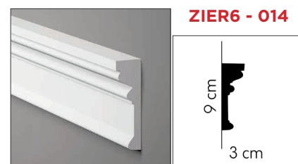
2000 x 30 x 90 mm / Polyurethan
