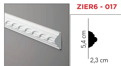
2000 x 23 x 54 mm / Polyurethan
