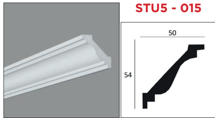
2000 x 54 x 50 mm / Polyurethan
