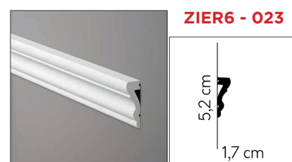
2000 x 17 x 52 mm / Polyurethan
