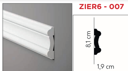
2000 x 19 x 81 mm / Polyurethan
