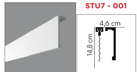
2000 x 46 x 148 mm / Polystyrol
