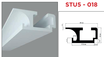
1150 x 250 x 120 mm / Polystyrol
