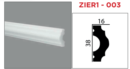
2000 x 15 x 40 mm / Polystyrol
