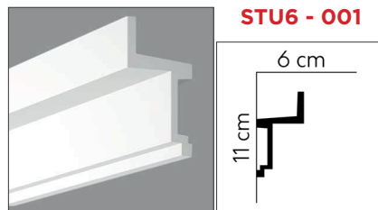
2000 x 60 x 110 mm / Profoam
