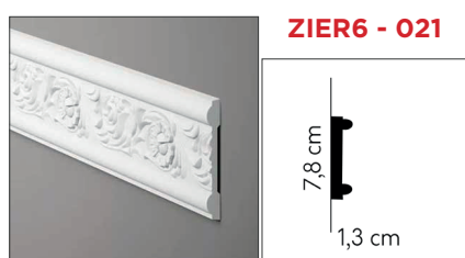
2000 x 13 x 78 mm / Polyurethan
