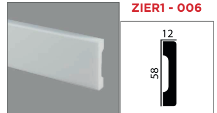
2000 x 12 x 58 mm / Polystyrol
