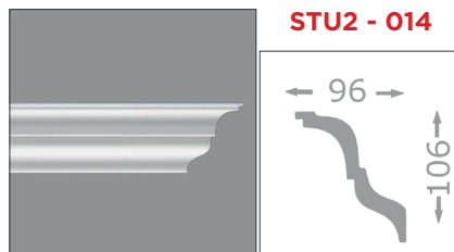
2000 x 96 x 106 mm / Polystyrol
