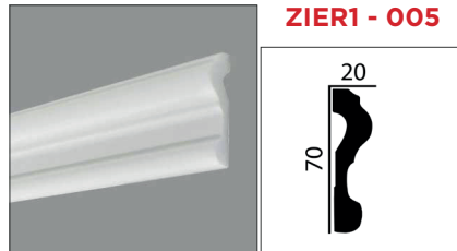
2000 x 20 x 70 mm / Polystyrol
