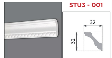
2000 x 32 x 32 mm / Polystyrol
