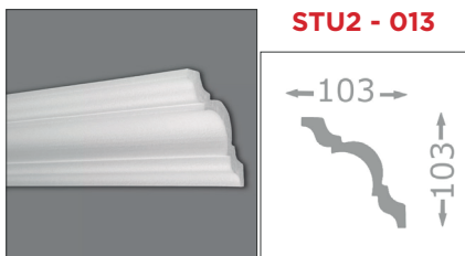
2000 x 103 x 103 mm / Polystyrol
