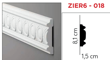
2000 x 15 x 81 mm / Polyurethan
