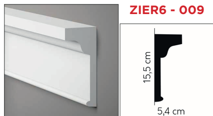
2000 x 54 x 155 mm / Polyurethan
