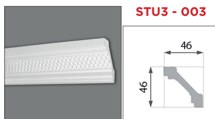
2000 x 46 x 46 mm / Polystyrol
