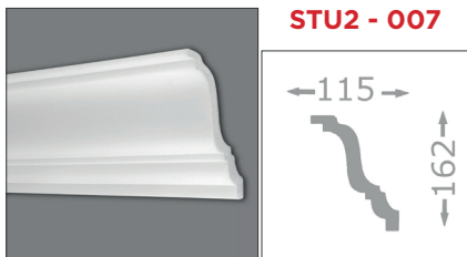
2000 x 115 x 162 mm / Polystyrol
