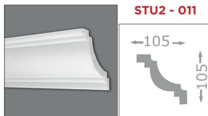
2000 x 105 x 105 mm / Polystyrol
