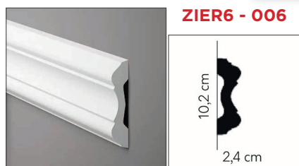
2000 x 24 x 102 mm / Polyurethan
