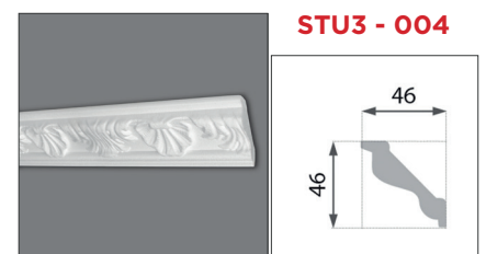
2000 x 46 x 46 mm / Polystyrol
