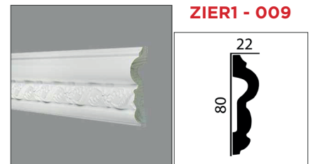
2000 x 20 x 80 mm / Polyurethan
