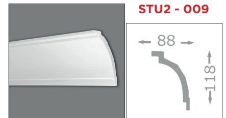
2000 x 88 x 118 mm / Polystyrol
