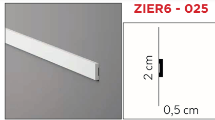
2000 x 5 x 20 mm / Polyurethan
