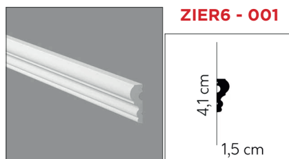
2000 x 15 x 41 mm / Polystyrol
