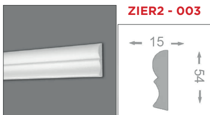
2000 x 15 x 54 mm / Polystyrol
