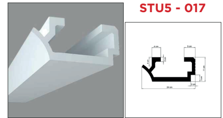
1150 x 240 x 110 mm / Polystyrol
