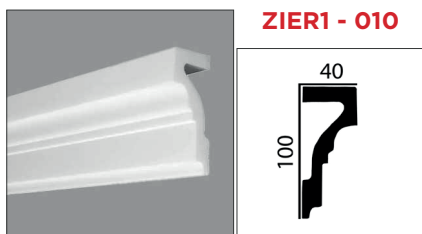
2000 x 40 x 100 mm / Polystyrol
