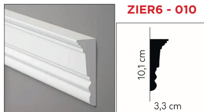
2000 x 33 x 101 mm / Polyurethan
