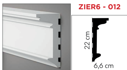
2000 x 66 x 220 mm / Polyurethan
