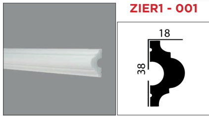
2000 x 20 x 40 mm / Polystyrol
