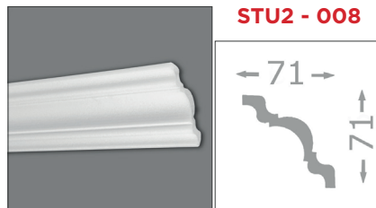
2000 x 71 x 71 mm / Polystyrol
