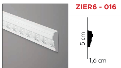
2000 x 16 x 50 mm / Polyurethan
