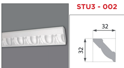
2000 x 32 x 32 mm / Polystyrol
