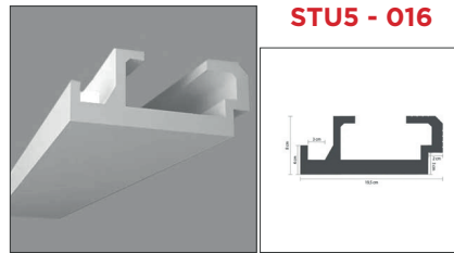
1150 x 195 x 80 mm / Polystyrol
